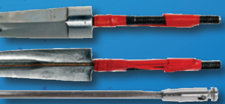
El. épée blade PBT-Ukraine Dynamo or STM
